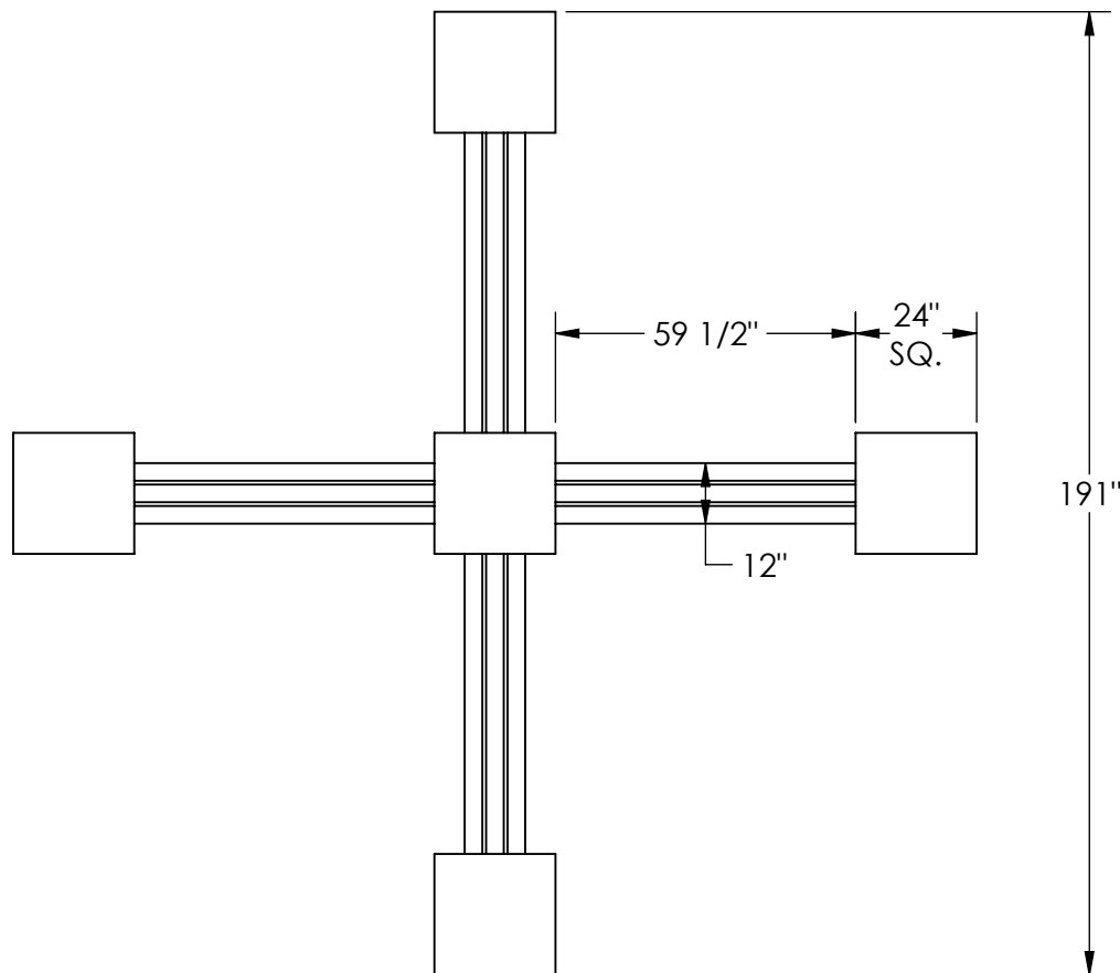
TOP VIEW
